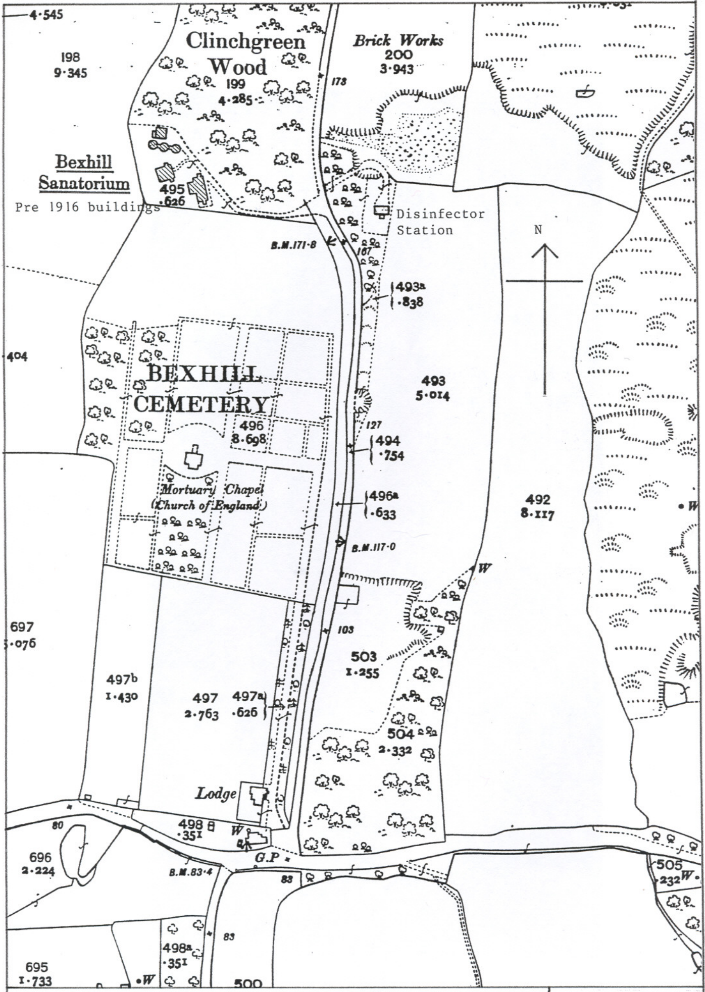
BEXHILL - ISOLATION HOSPITAL ST MARY'S LANE NGR TQ 72630971 Site Plan from 1:2500 OS 1910 edition
